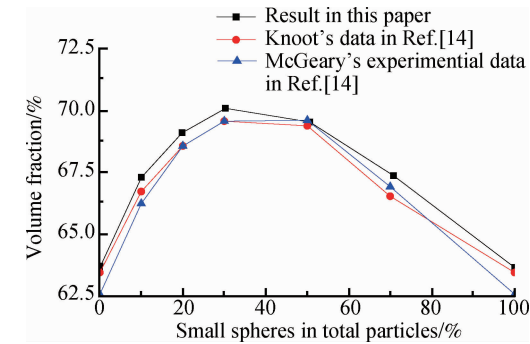
图 1 颗粒最大体积分数试验及仿真结果 Fig. 1 Results of particles' maximum volume fraction from experiment and simulations
